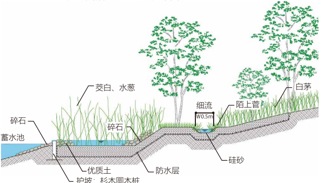
b-b' section
